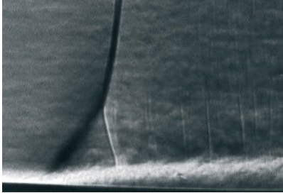
Schlieren photograph (density gradient) of the flow above an airfoil at Mach 0.9.
