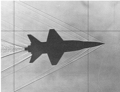
Schlieren photograph of Mach waves and oblique shockwaves around a supersonic aircraft.
